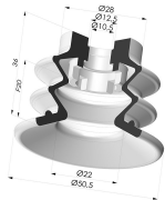
Sauggreifer 2.5 Falten Serie 96C Ø 50MM
