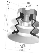
Sauggreifer 2.5 Falten Serie 96C Ø 50MM
