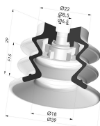
Sauggreifer 2.5 Falten Serie 96C Ø 40MM
